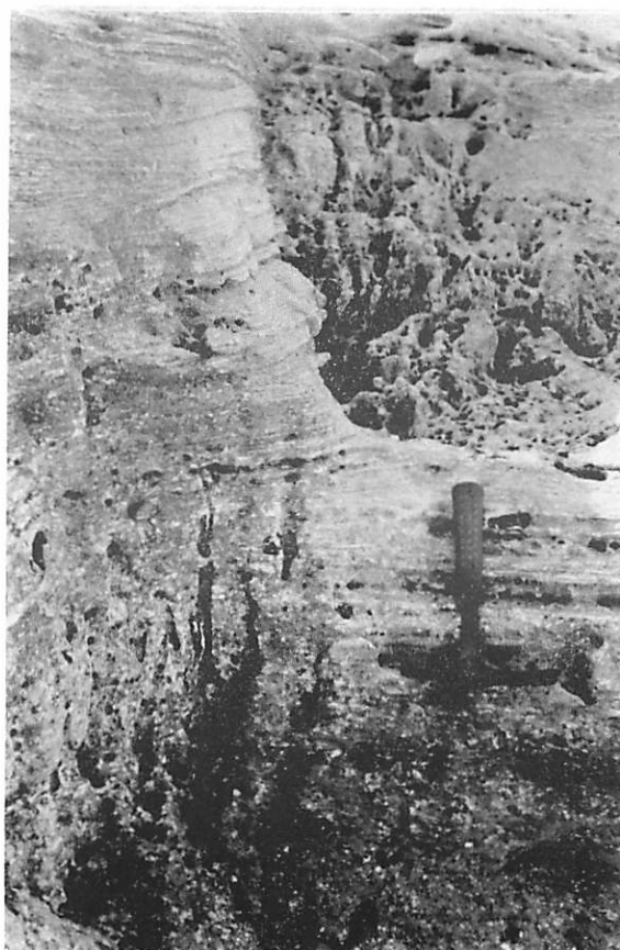
Fig. 11. Two examples of cluster burrows in the lower part of the sequence at the Salt Pond Dune locality. One cluster to the left of the hammer the other one above it.
