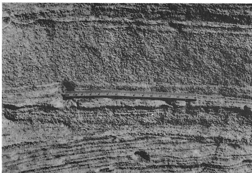
Fig. 10. A layer of grainfall deposits between climbing wind ripple laminations at the Salt Pond Dune locality. Scale in centimeters.
