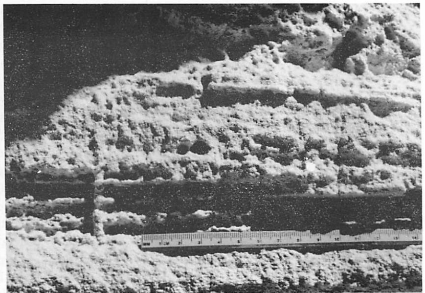
Fig. 8. Skolithos in eolianites (to the left of the scale) at the Dune Pass Lobe locality. Scale in centimeters.
