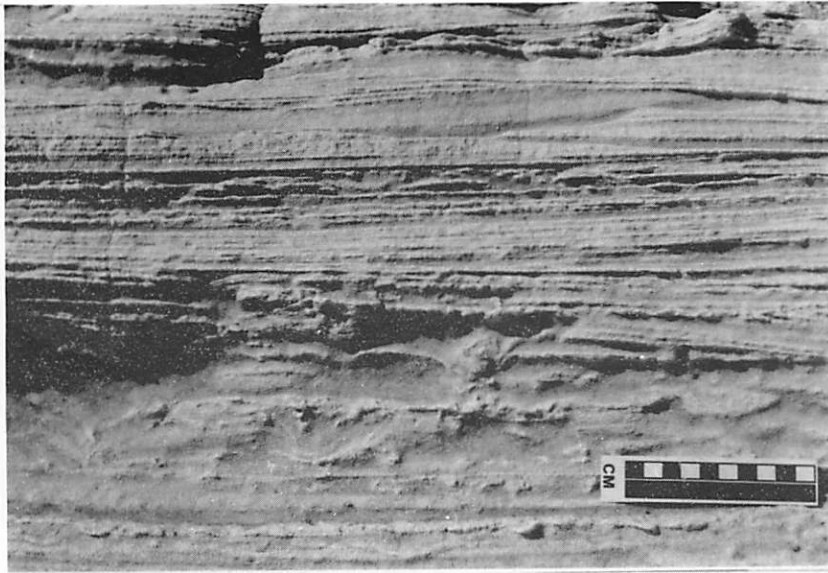
Fig. 6. Climbing wind ripple laminations and layers with small, irregular burrows in eolianites at the Dune Pass Lobe locality. Note prominent bioturbation to the left of the scale.
