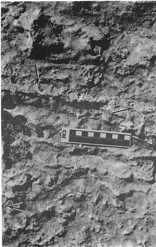
Fig. 7. Bioturbation of eolianites by small, irregular burrows at the Dune Pass Lobe locality. Arrows point to examples of burrows with pale walls. Compare with the well preserved laminations and lee-side structures shown in Fig. 5.
