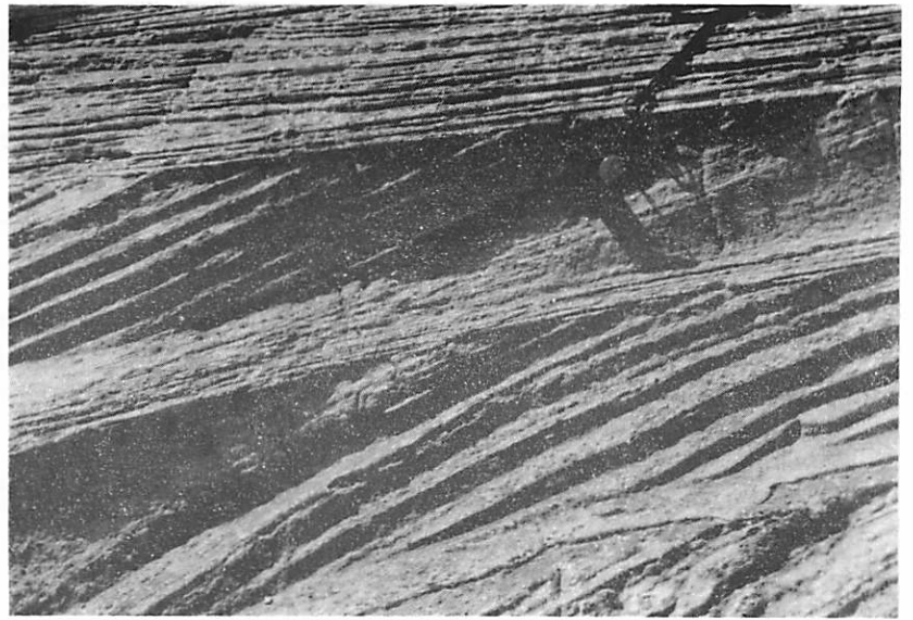
Fig. 5. Climbing wind ripple laminations and lee-side sandflow deposits in eolianites at the Dune Pass Lobe locality. Hand lens for scale.
