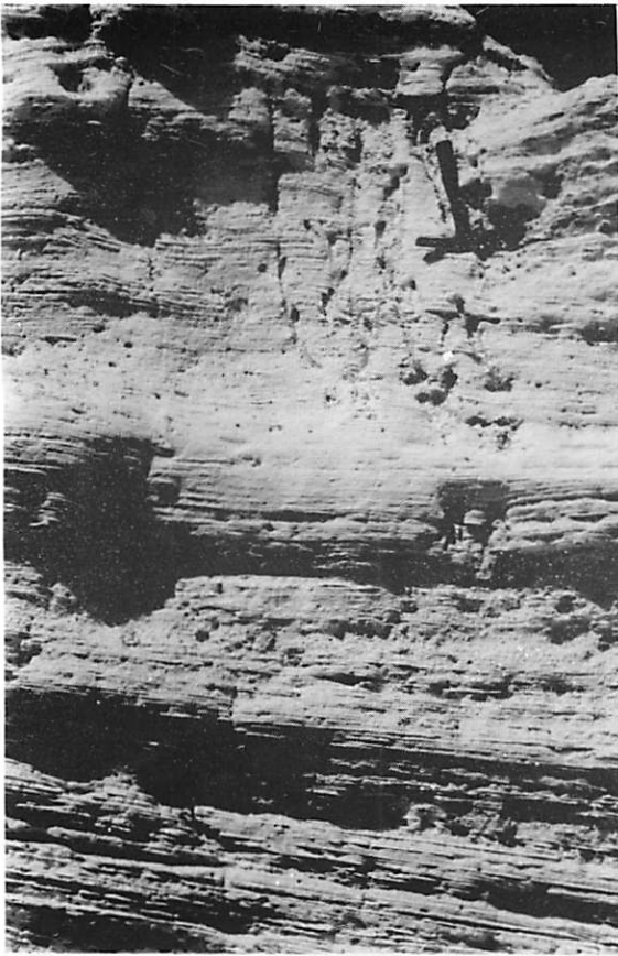
Fig. 12. An example of a cluster burrow (to the left of the hammer) in the upper part of the sequence at the Salt Pond Dune locality.
