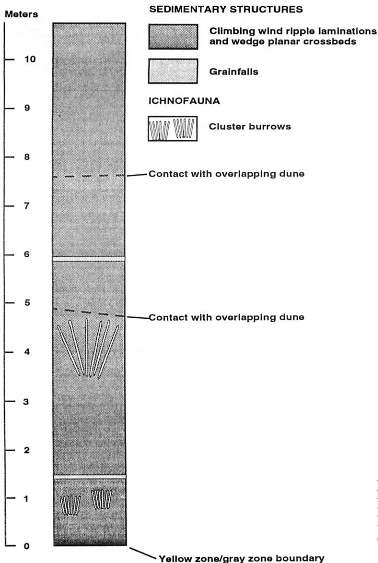
Fig. 9. Stratigraphic sequence at the Salt Pond Dune locality.
