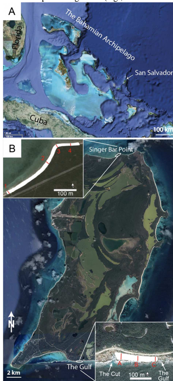
Figure 1. Study area. A) The Bahama Archipelago, with Florida and Cuba for context, and San Salvador Island. B) Map of San Salvador with the two study sites labeled: Singer Bar Point (SBP) along the relatively low-energy north coast, and The Gulf (TG) on the high-energy south coast. Insets show the study sites outlined in white, with red lines and labels marking the location of profiles shown in Figure 2 (source: Google Earth).
