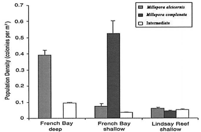
Figure 4 Population density of millepores separated by depth and specific reef. Error bars represent standard error of the mean. Shallow = 1-3m and deep > 3m. Data shown are from French Bay and Lindsay Reef. N (number of transects) = 19 for French Bay deep, N = 24 for French Bay shallow, and N = 10 for Lindsay Reef.
