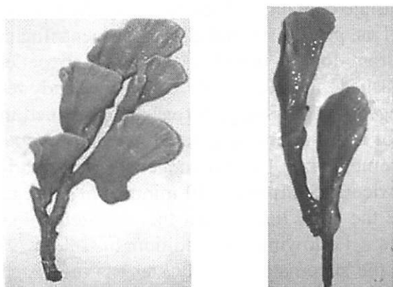
Figure 2. Photographs depicting examples of intermediate growth forms of Millepora found around San Salvador Island, Bahamas.
