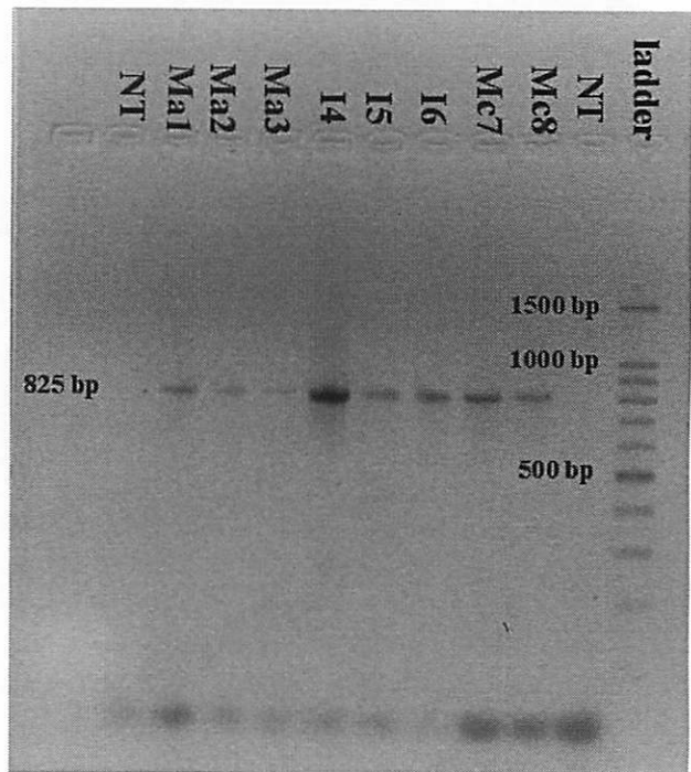
Figure 6. PCR amplification of rDNA using the A18S/ITS 4 primers. The single band corresponds to a size of approximately 825 base pairs. Ma = M. alcornis (branched growth form), I = intermediate and Mc = M. complanata (bladed growth form). The number following the sample name denotes the sample number. NT = no template controls and a 100 base pair ladder is shown.
