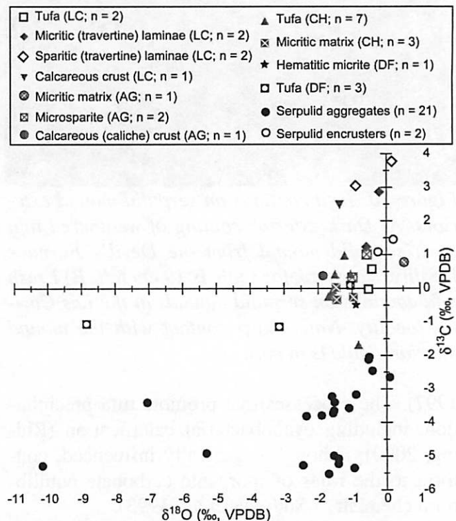
Figure 13. Stable isotope composition of tufa and various associated carbonate components from the Dominican Republic. Study sites: LC-Las Caritas; CH-Cañada Honda; AG-Abuela Grande; DF-Devil's Furnace (see Figure 1B).
